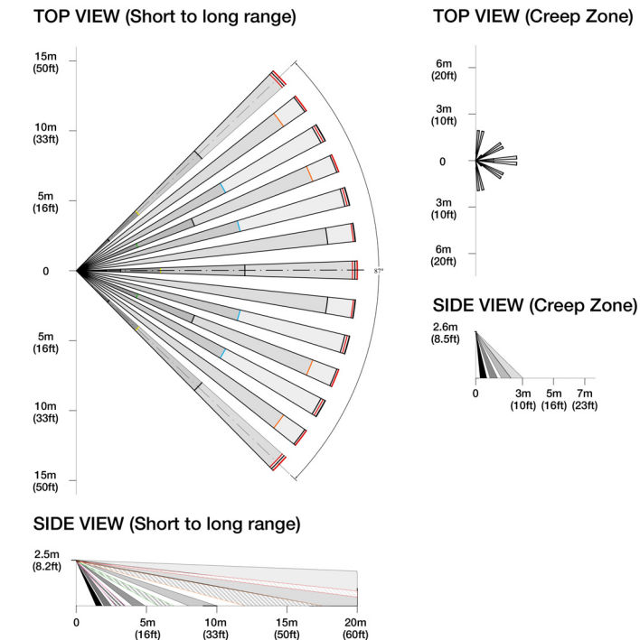
Figure 1: Beam Patterns
